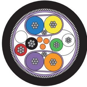
USB 3.2 Gen 2 – 1D.310 configuration
