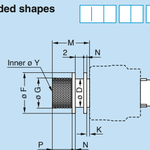
Heatshrink molded shapes
